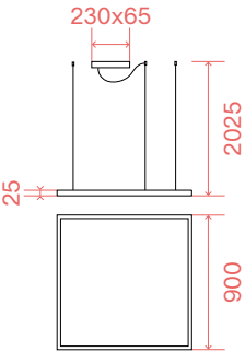
LED SMD (DRIVER ON/OFF INCLUDED)
